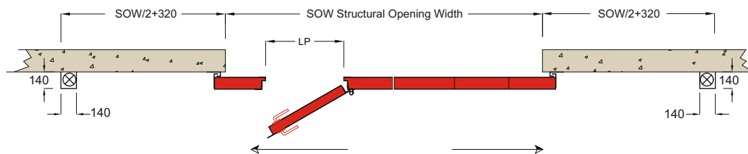
SEC. A - A'
